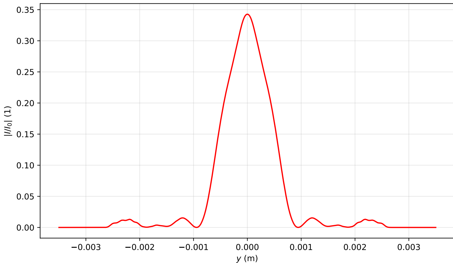
Intensity profile I(x=0, y, z=0.955)/I_0 , \text{Pin}=3.0\text{Pcr} , artificial time
